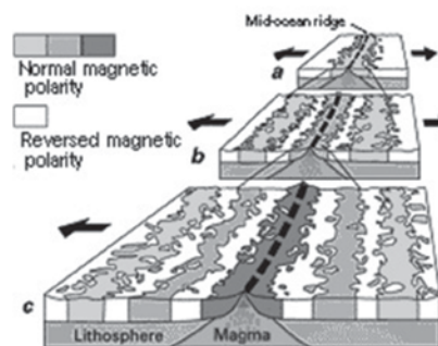
The Spreading Ocean Floor
