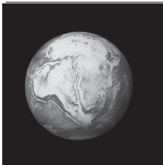
Africa & South America fit together like puzzle pieces
